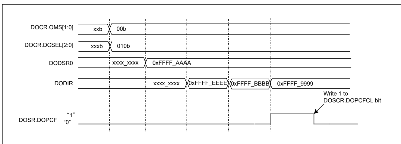
Figure 58.4 Example of Operation in Data Comparison Mode (Detection condition: Lower)
